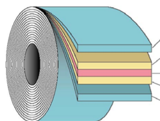
PE coated paper Solvent based pure Acrylic adhesive PET film 12µ Solvent based pure Acrylic adhesive PE coated paper
