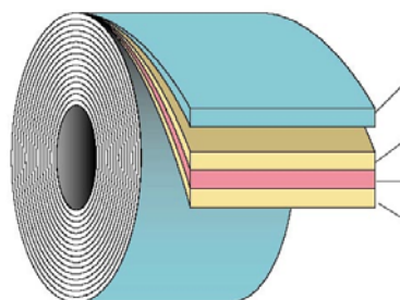
Siliconised white paper Side 2: Solvent based modified acrylic adhesive White PE Foam 1,0 mm Side 1: Solvent based modified acrylic adhesive
